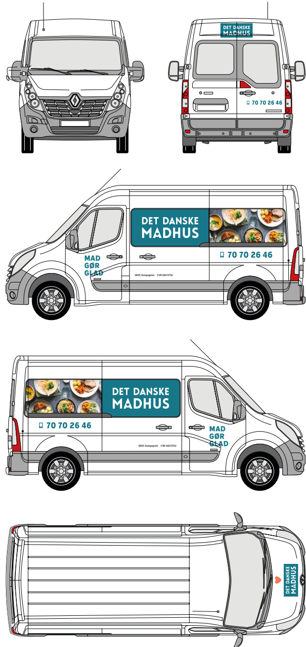
Rena_596 | Copyright by creativ collection Verlag GmbH, Germany | www.cvision.de Renault Master, L2H2, FWD, 2 Schiebetuere, Heck verglast (2014) 1:30 L: 5.548 B: 2.070 H: 2.500 R: 3.682
