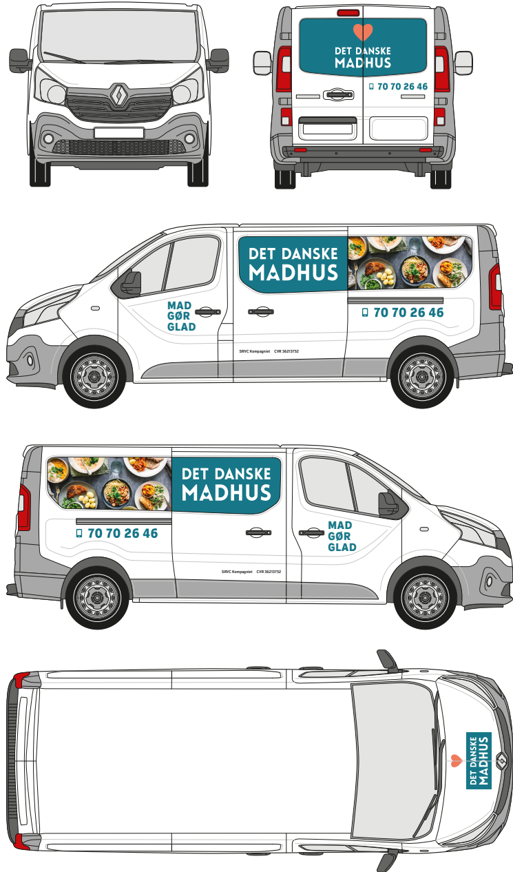
Rena_562 | Copyright by creativ collection Verlag GmbH, Germany | www.cvision.de Renault Trafic Kasten, L2H1, Heckfluegelt., 2 Schiebet. (2014) 1:30 L: 5.399 B: 1.956 H: 1.971 R: 3.498
